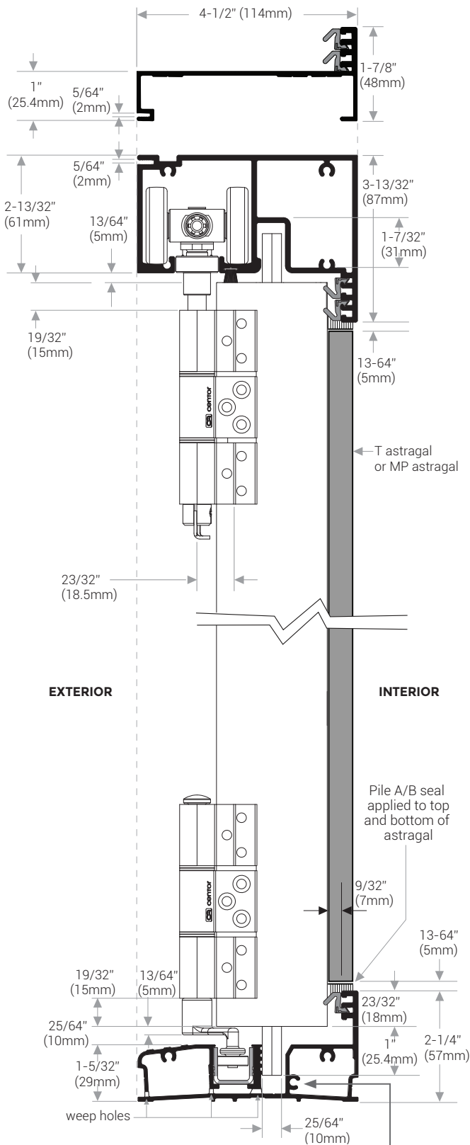
Panel to Sill Detail
